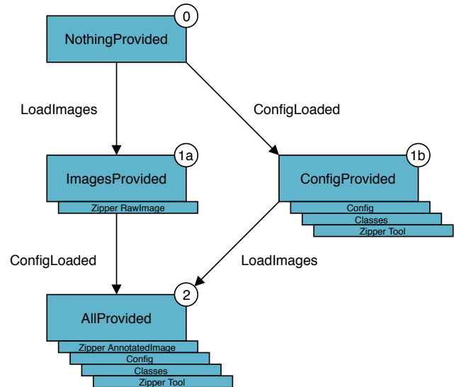
Figure 4: The application states.
