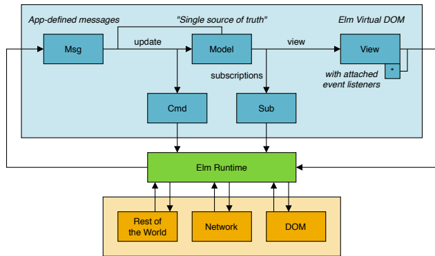
Figure 3: The application architecture.
